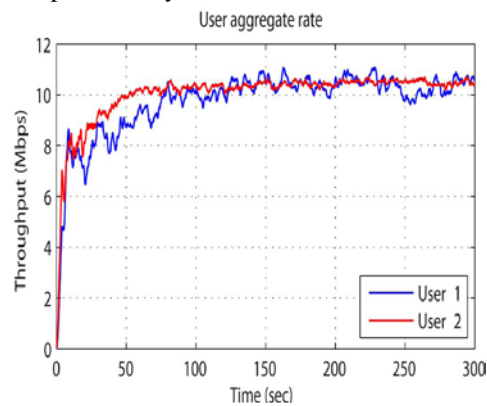
Fig 3:Result for Controlling the Number of Connections
