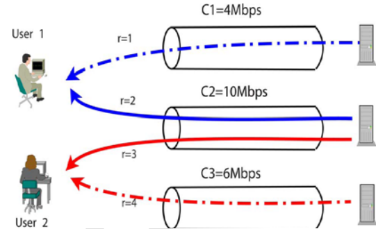
Fig 2: Marginal utility with route price
